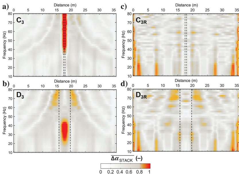
Figure 10. Stacked attenuation coefficient results on (a) C 3 , (b) D 3 , (c) C 3R , and (d) D 3R . In each section, the vertical dashed lines highlight the real position of the lateral variations.
