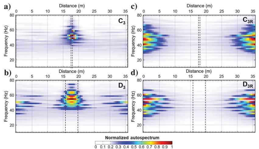
Figure 13. Multifold stacked autospectrum results on (a) C_3 , (b) D_3 , (c) C_{3R} , and (d) D_{3R} . In each section, the vertical dashed lines highlight the real position of the lateral variations.
