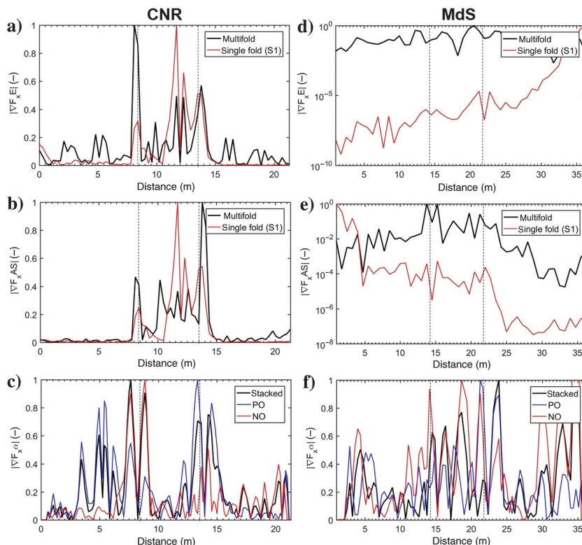
Figure 23. Comparison of single-fold/offset and stacked results for the field data (a-c) CNR and (d-f) Madonna del Sasso. (a and d) S1 and multifold stacked normalized energy gradients. (b and e) S1 and multifold stacked normalized autospectrum gradients. (c and f) Attenuation coefficient normalized gradients for positive offset (PO), negative offset (NO), and stacked results. In (d and e), the y-axis is in logarithmic scale to intensify the small fluctuations of single-fold gradients.
