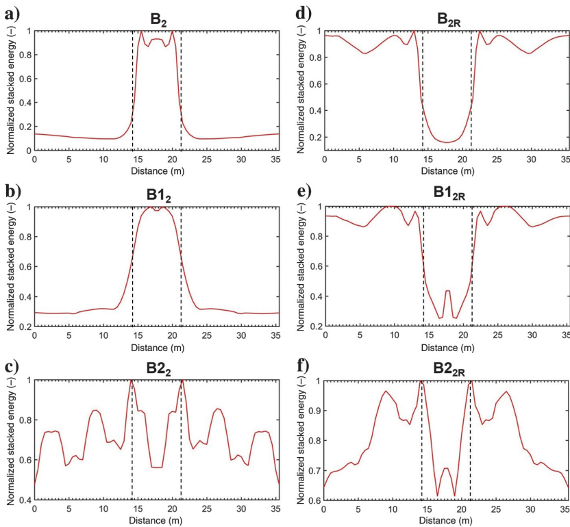
Figure 3. Multifold stacked energy results. (a) B 2 , (b) B 12 , (c) B 22 , (d) B 2R , (e) B 12R , and (f) B 22R . In each section, the vertical dashed lines highlight the real position of the lateral variations.
