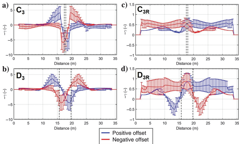
Figure 7. Energy decay exponent results on (a) C_3 , (b) D_3 , (c) C_{3R} , and (d) D_{3R} . In each section, the vertical dashed lines highlight the real position of the lateral variations.
