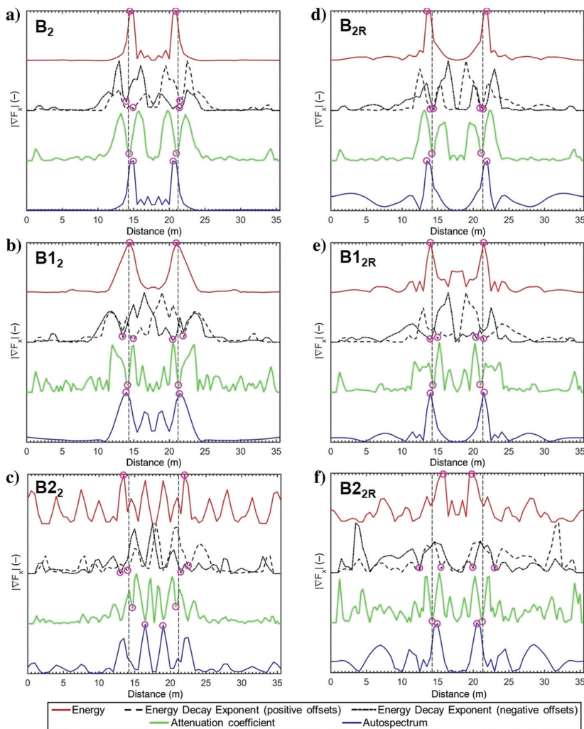
Figure 19. Normalized absolute value of the horizontal gradients of the four parameters on (a) B_2 , (b) B_{12} , (c) B_{22} , (d) B_{2R} , (e) B_{12R} , and (f) B_{22R} synthetic models: energy (in red), energy decay exponent (in black; dashed line: positive offsets; dashed-dotted line: negative offsets), attenuation coefficient (in green), and autospectrum (in blue). In each section, the vertical dashed lines mark the real position of the lateral variations, whereas the magenta circles highlight the locations of the lateral variations, according to the criteria described in the text.
