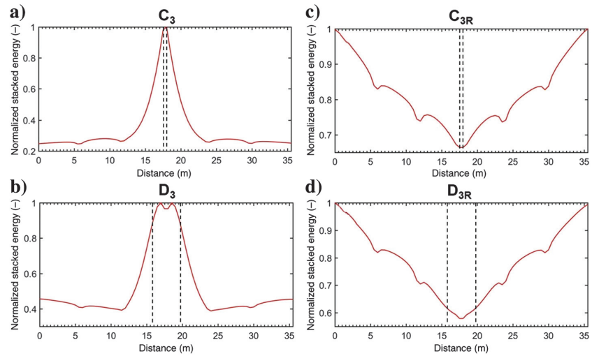
Figure 4. Multifold stacked energy results. (a) C_3 , (b) D_3 , (c) C_{3R} , and (d) D_{3R} . In each section, the vertical dashed lines highlight the real position of the lateral variations.
