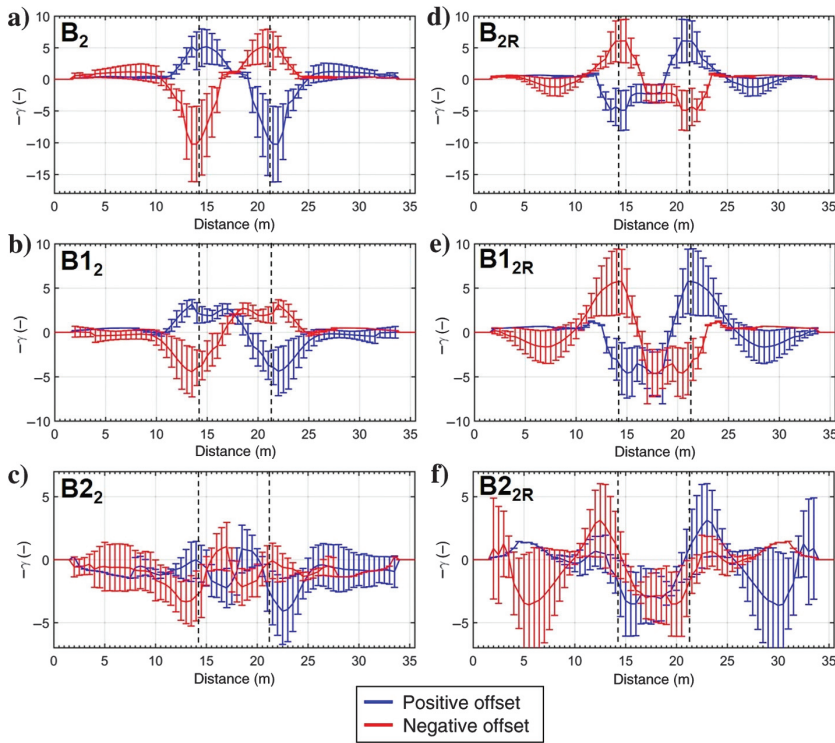
Figure 6. Energy decay exponent results on (a) B_2 , (b) B_{1_2} , (c) B_{2_2} , (d) B_{2R} , (e) B_{1_{2R}} , and (f) B_{2_{2R}} . In each section, the vertical dashed lines highlight the real position of the lateral variations.
