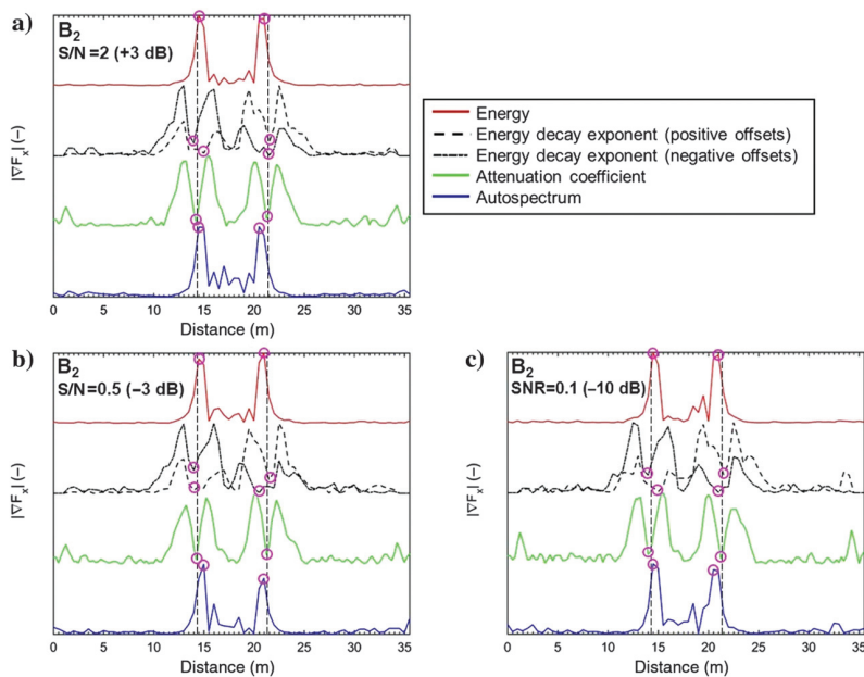
Figure B-3. Normalized absolute value of the horizontal gradients of the four parameters on the perturbed model B_2 (a) S/N = 2 , (b) S/N = 0.5 , and (c) S/N = 0.1 : energy (in red), energy decay exponent (in black; dashed line: positive offsets; dashed-dotted line: negative offsets), attenuation coefficient (in green), and autospectrum (in blue). In each section, the vertical dashed lines mark the real position of the lateral variations, whereas the magenta circles highlight the locations of the lateral variations, according to the adopted criteria.
