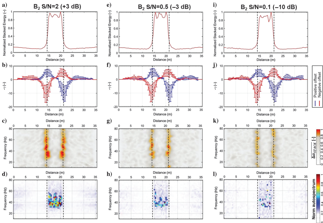
Figure B-2. Results on the perturbed model B_2 (a-d) S/N = 2 , (e-h) S/N = 0.5 , and (i-l) S/N = 0.1 . (a, e, and i) Multifold stacked energy plots. (b, f, and j) Energy decay exponent results. (c, g, and k) Stacked attenuation coefficient plots. (d, h, and l) Multifold stacked autospectrum plots.
