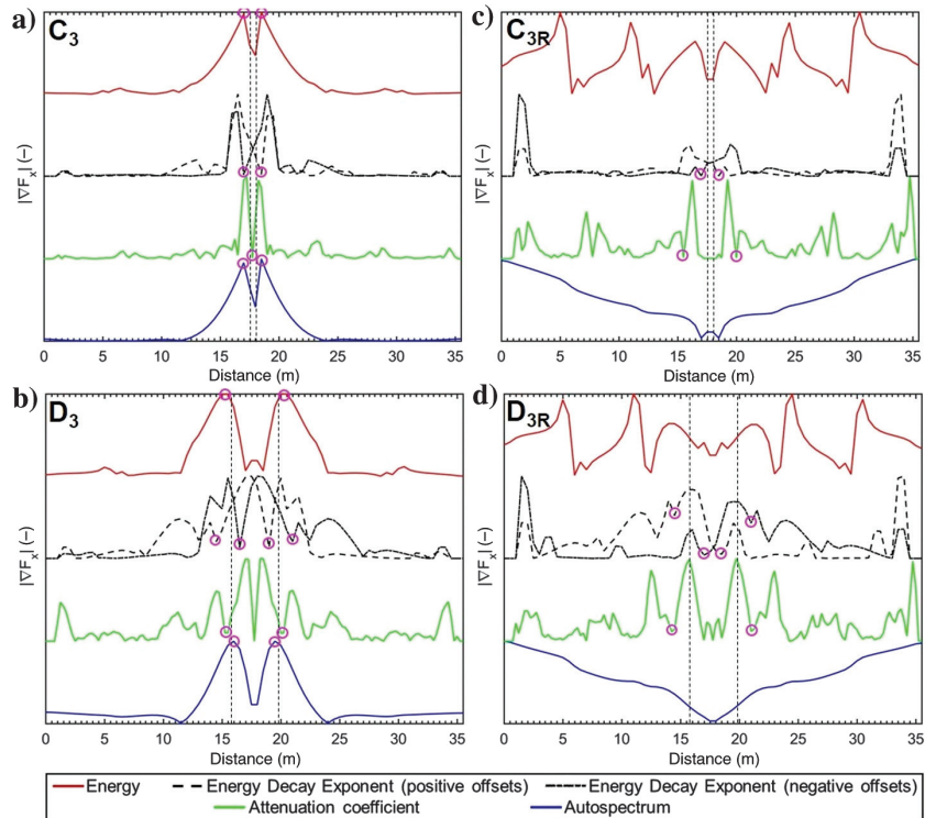
Figure 20. Normalized absolute value of the horizontal gradients of the four parameters on (a) C_3 , (b) D_3 , (c) C_{3R} , and (d) D_{3R} : energy (in red), energy decay exponent (in black; dashed line: positive offsets; dashed-dotted line: negative offsets), attenuation coefficient (in green), and autospectrum (in blue). In each section, the vertical dashed lines mark the real position of the lateral variations, whereas the magenta circles highlight the locations of the lateral variations, according to the criteria described in the text.
