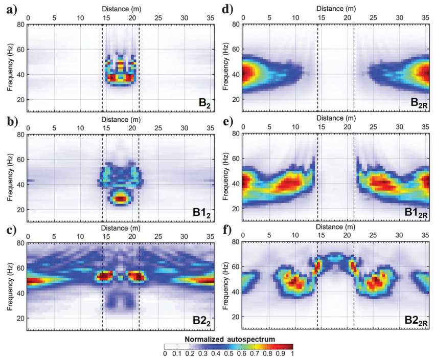
Figure 12. Multifold stacked autospectrum results on (a) B_2 , (b) B_{1_2} , (c) B_{2_2} , (d) B_{2R} , (e) B_{1_{2R}} , and (f) B_{2_{2R}} . In each section, the vertical dashed lines highlight the real position of the lateral variations.
