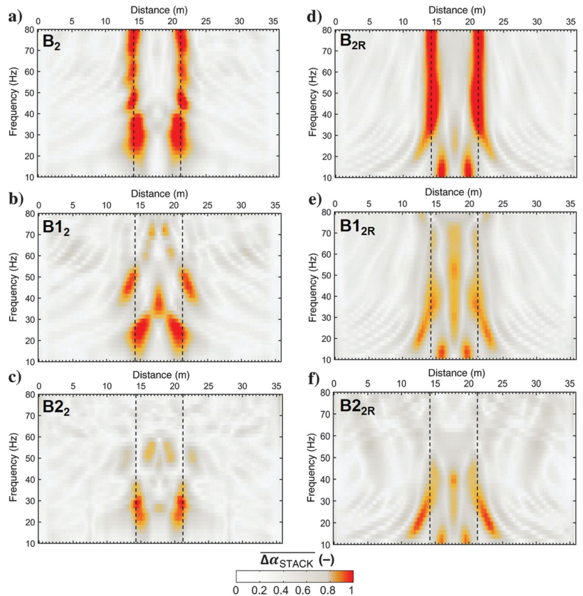
Figure 9. Stacked attenuation coefficient results on (a) B_2 , (b) B_{1_2} , (c) B_{2_2} , (d) B_{2_R} , (e) B_{1_{2R}} , and (f) B_{2_{2R}} . In each section, the vertical dashed lines highlight the real position of the lateral variations.
