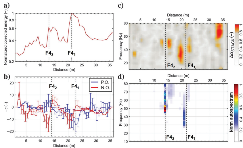
Figure 17. Madonna del Sasso results. (a) Multifold stacked energy-distance plot. (b) Energy decay exponent results. (c) Stacked attenuation coefficient results. (d) Multifold stacked autospectrum plot. In each section, the vertical dashed lines highlight the approximate real position of the fractures.
