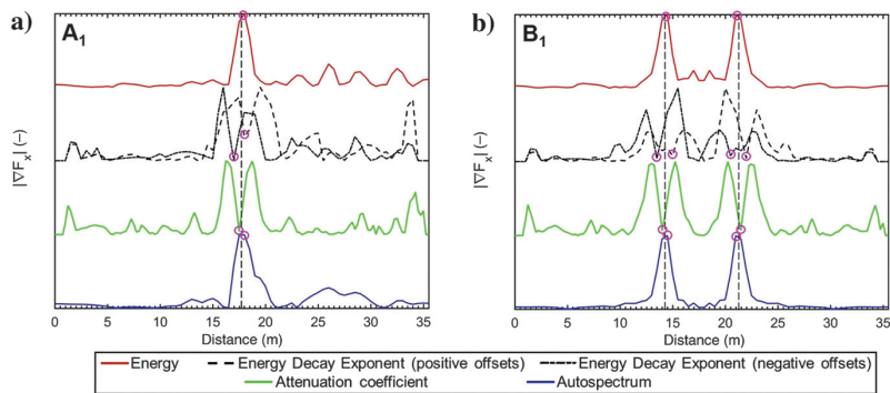
Figure 18. Normalized absolute value of the horizontal gradients of the four parameters on the (a) A_1 and (b) B_1 synthetic models: energy (in red), energy decay exponent (in black; dashed line: positive offsets; dashed-dotted line: negative offsets), attenuation coefficient (in green), and autospectrum (in blue). In each section, the vertical dashed lines mark the real position of the lateral variations, whereas the magenta circles highlight the locations of the lateral variations, according to the criteria described in the text.
