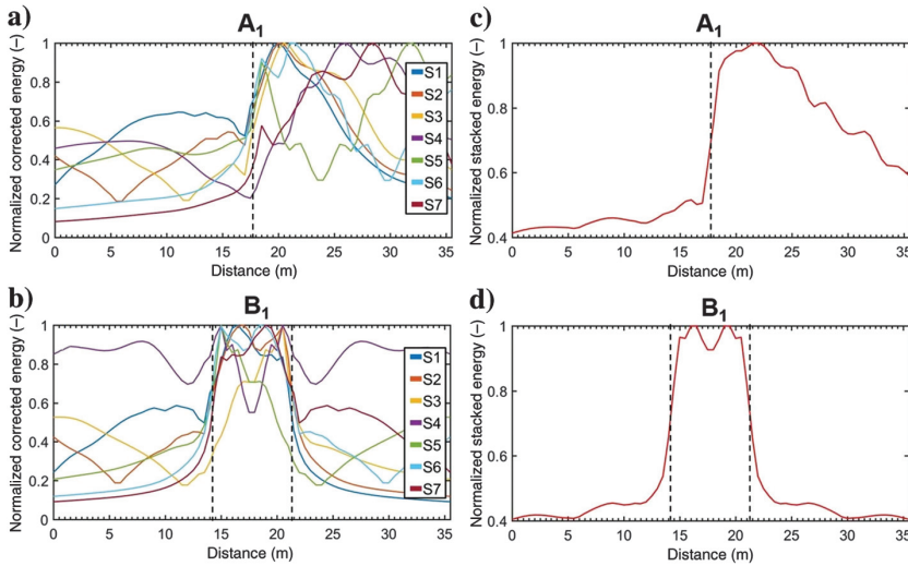
Figure 2. Energy results on (a and c) A 1 and (b and d) B 1 . Left column: single-fold results; right column: multifold stacked results. In each section, the vertical dashed lines highlight the real position of the lateral variations.
