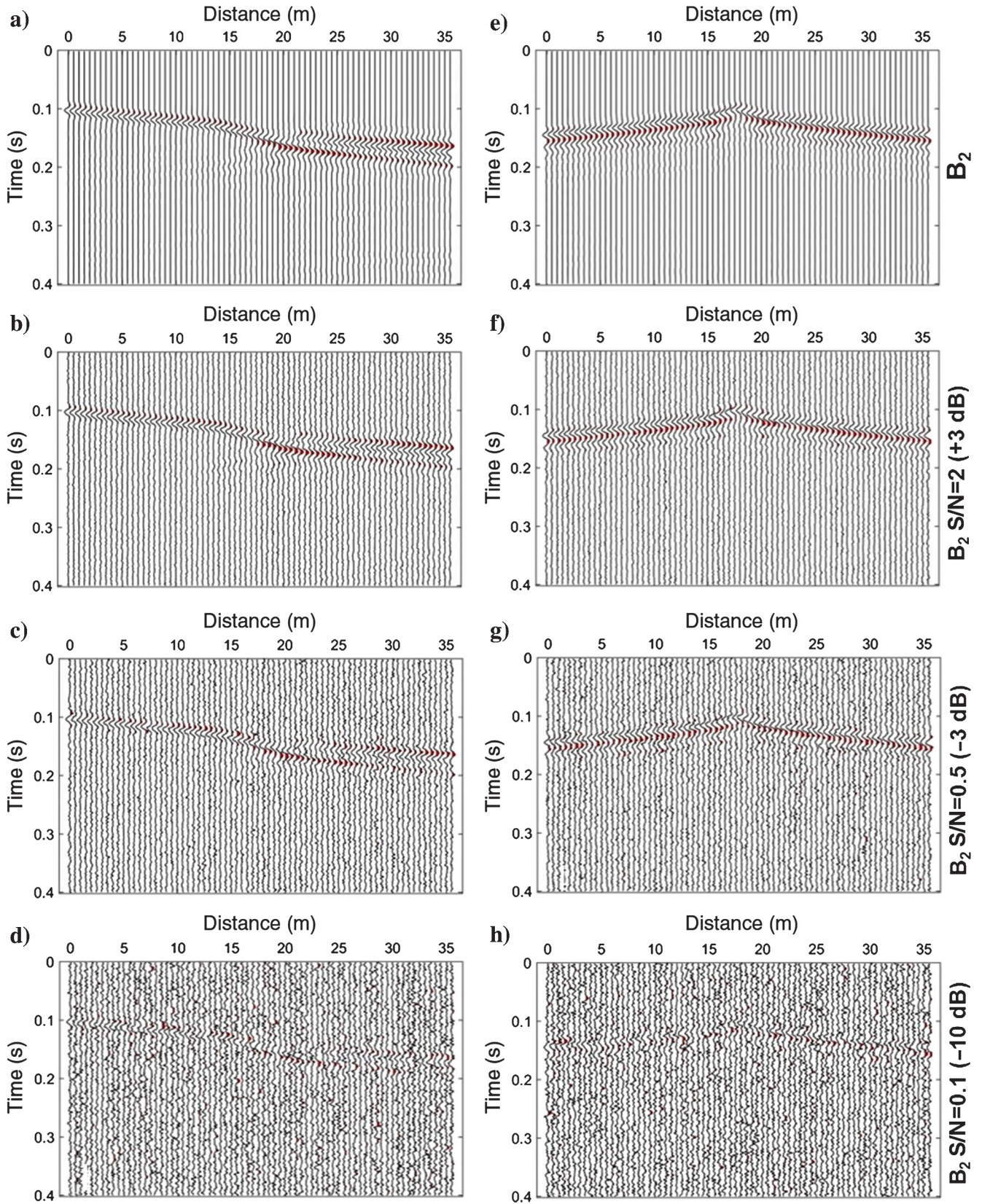
Figure B-1. Synthetic CSGs for model B_2 . (a-d) S1 and (e-h) S4. (a and e) Unperturbed traces, (b and f) S/N = 2 , (c and g) S/N = 0.5 , and (d and h) S/N = 0.1 .
