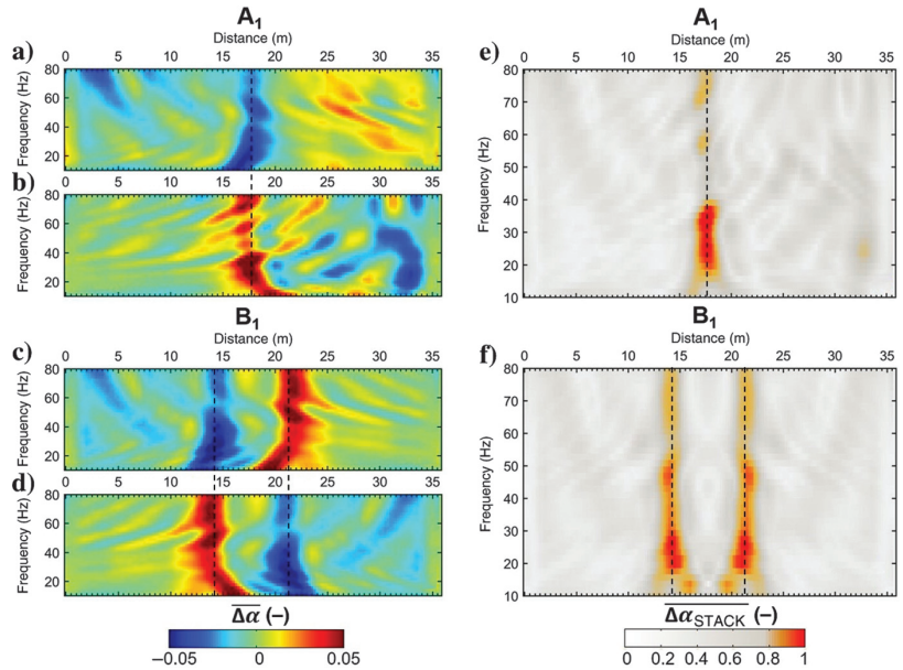
Figure 8. Attenuation coefficient results on (a, b, and e) A_1 and (c, d, and f) B_1 . Left column: separate plots for positive (top) and negative (bottom) offsets. Right column: stacked plot of the single-offset plots (absolute value) on the left. In each section, the vertical dashed lines highlight the real position of the lateral variations.
