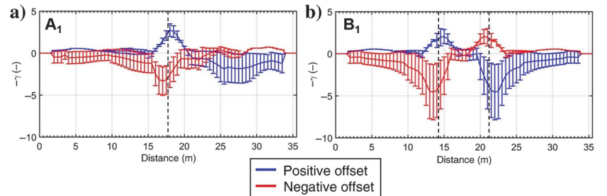
Figure 5. Energy decay exponent results on (a) A_1 and (b) B_1 . In each section, the vertical dashed lines highlight the real position of the lateral variations.
