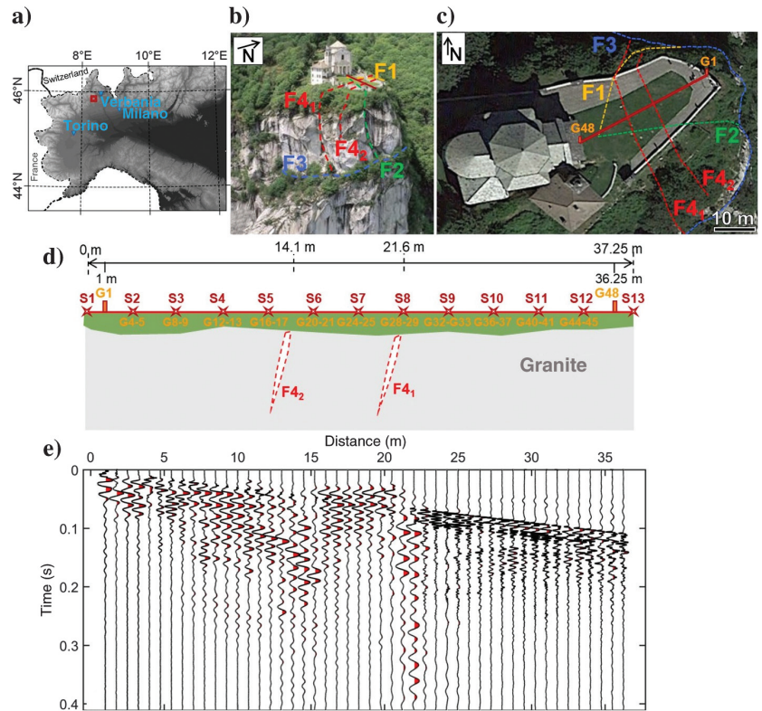
Figure 16. Madonna del Sasso test site. (a) Geographic location. (b and c) Aerial views of the site with location of the main fractures (F1 to F4, dashed lines) and seismic array (the red continuous line). (d) Geometry of the seismic layout and fracture locations. G1–G48: geophone locations; S1–S13: shot locations. (e) CSG for S1.
