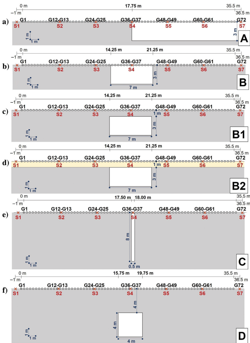
Figure 1. Geometries adopted for the synthetic models, reproducing different shapes of the heterogeneities and embedment conditions. The model parameters are summarized in Table 1 (the model name and subscript refer to geometry and material parameters, respectively). (a) A_1 , (b) B_1 , B_2 , and B_{2R} , (c) B_{12} and B_{12R} , (d) B_2 and B_{2R} , (e) C_3 and C_{3R} , and (f) D_3 and D_{3R} . G1–G72: geophone locations; S1–S7: shot locations.
