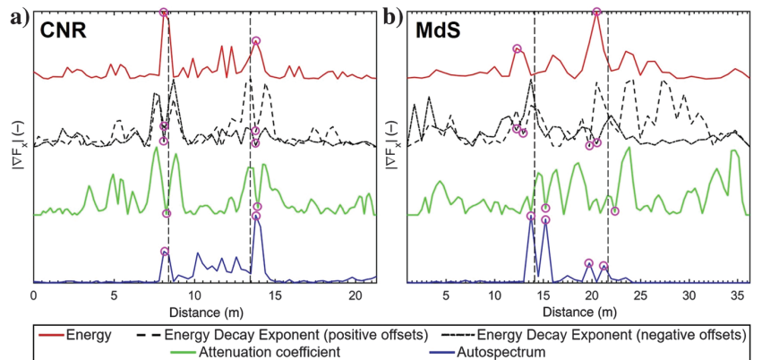
Figure 21. Normalized absolute value of the horizontal gradients of the four parameters on (a) CNR test site and (b) Madonna del Sasso cliff: energy (in red), energy decay exponent (in black; dashed line: positive offsets; dashed-dotted line: negative offsets), attenuation coefficient (in green), and autospectrum (in blue). In each section, the vertical dashed lines mark the real position of the lateral variations, whereas the magenta circles highlight the locations of the lateral variations, according to the criteria described in the text.
