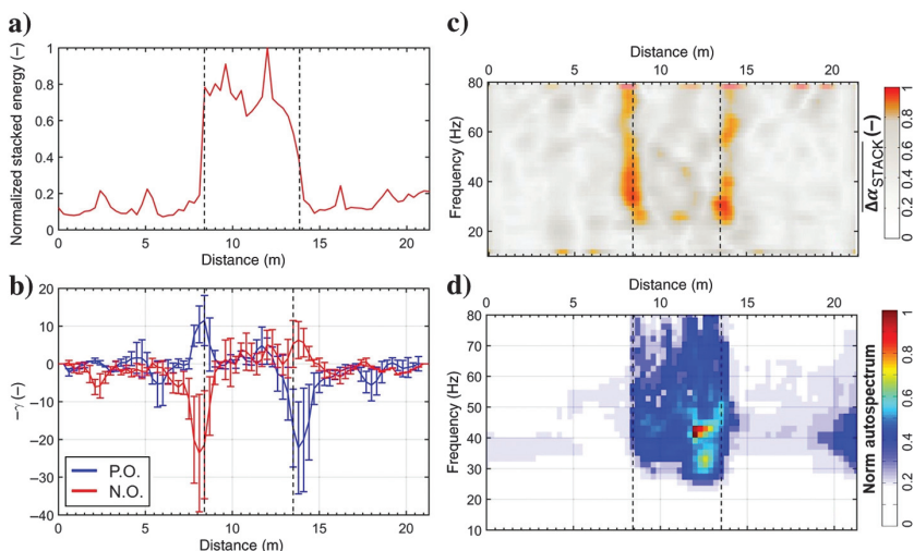
Figure 15. The CNR results. (a) Multifold stacked energy-distance plot. (b) Energy decay exponent results. (c) Stacked attenuation coefficient results. (d) Multifold stacked autospectrum plot. In each section, the vertical dashed lines highlight the approximate real position of the box edges.
