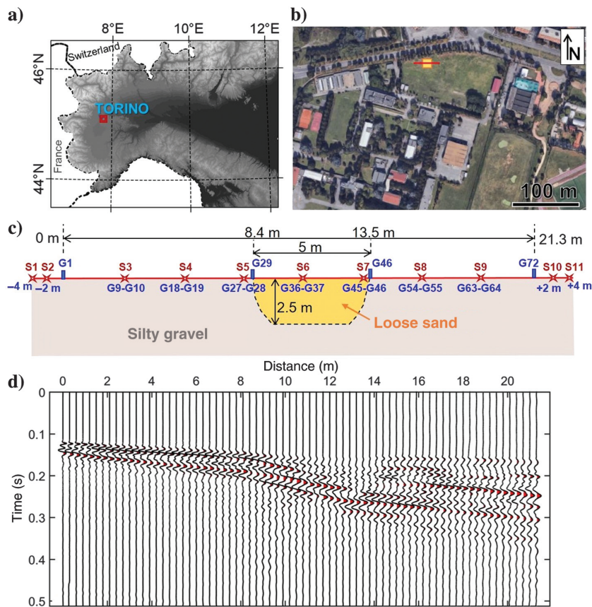
Figure 14. The CNR test site. (a) Geographic location. (b) Aerial view of the site with location of the sand box (the yellow square) and the seismic array (the red line). (c) Geometry of the target and seismic layout. G1–G72: geophone locations; S1–S11: shot locations. (d) CSG for S1.
