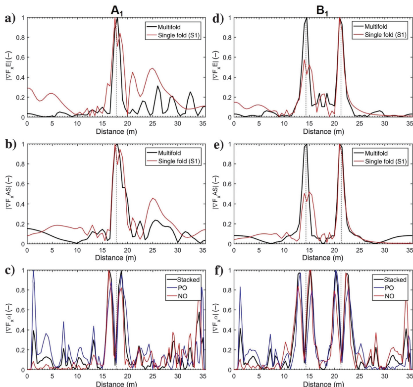
Figure 22. Comparison of single-fold/offset and stacked results for the synthetic model (a-c) A 1 and (d-f) B 1 . (a and d) S1 and multifold stacked normalized energy gradients. (b and e) S1 and multifold stacked normalized autospectrum gradients. (c and f) Attenuation coefficient normalized gradients for the positive offset, negative offset, and stacked results.
