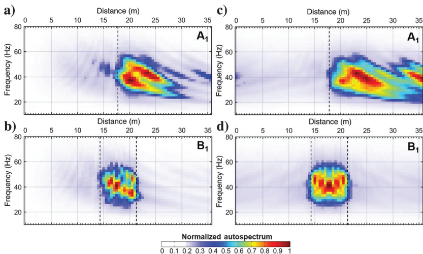
Figure 11. Autospectrum results on (a and c) A 1 and (b and d) B 1 . Left column: single-fold autospectrum of shot S1. Right column: multifold stacked autospectrum. In each section, the vertical dashed lines highlight the real position of the lateral variations.
