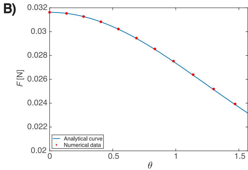
Figure 2 Numerical simulation of single tape peeling A) 3D displacement map. The colormap indicates the z displacement. B) Numerical vs. analytical prediction of pull-off force vs peeling angle.
