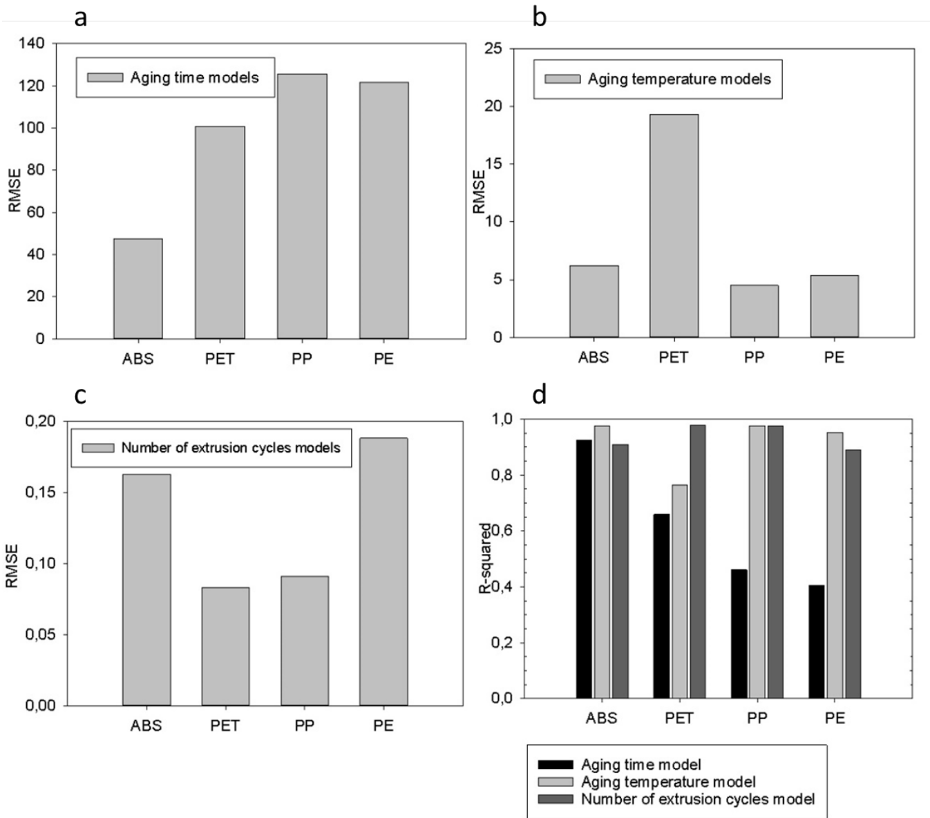
Figure 6. Evaluation of the global aging models for ABS, PET, PP and PE; (a) RMSE for the aging time component, (b) RMSE for the aging temperature component, (c) RMSE
