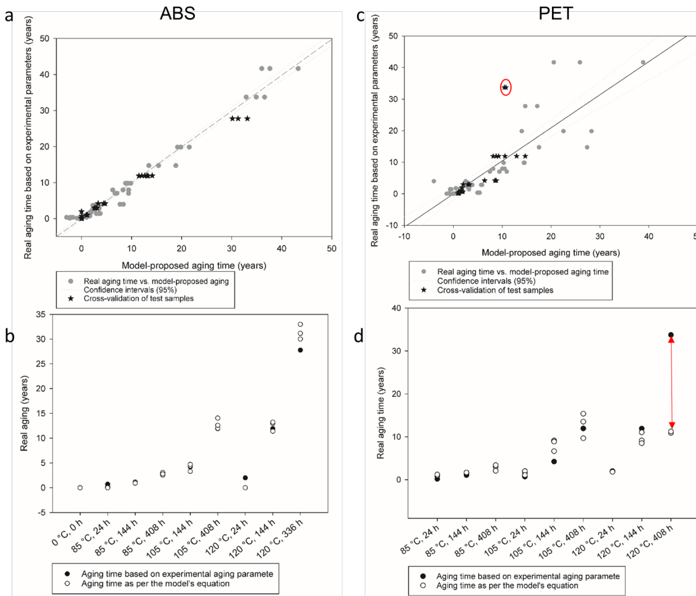
Figure 2. Left (a, b) for ABS and right (c, d) for PET: (a, c) Test samples cross-validated with the aging model, (b, d) comparison between real thermo-oxidative aging time obtained from experimental parameters and real thermo-oxidative aging time obtained from the generated regression model.
