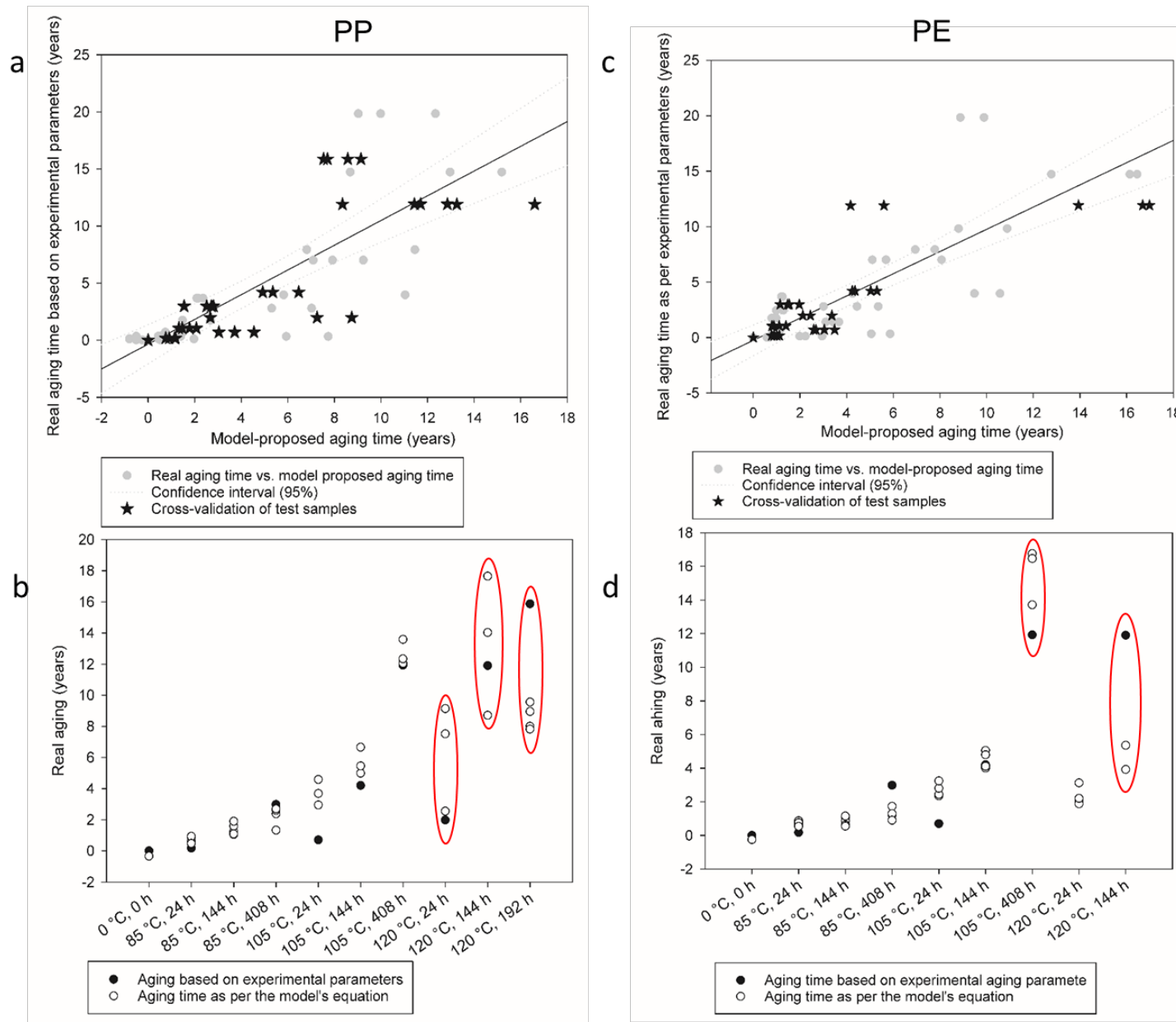
Figure 3. Left (a, b) for PP and right (c, d) for PE: (a, c) test samples cross-validated with the aging model, (b, d) comparison between real thermo-oxidative aging time obtained from experimental parameters and real thermo-oxidative aging time obtained from the generated regression model.
