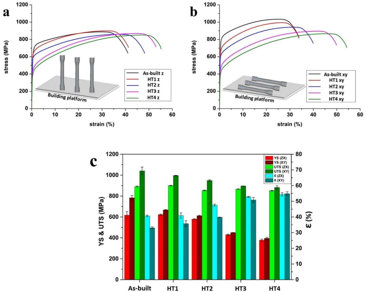
Figure 9 - Representative plots of tensile stress-strain diagrams of as-built and heat-treated specimens: (a) along the building direction (z-axis); (b) perpendicular to the building direction (xy plane); (c) Plots of the YS, UTS and \epsilon recorded by LPBF IN625 tensile specimens in the as-built and heat-treated states along z-axis and xy plane.
