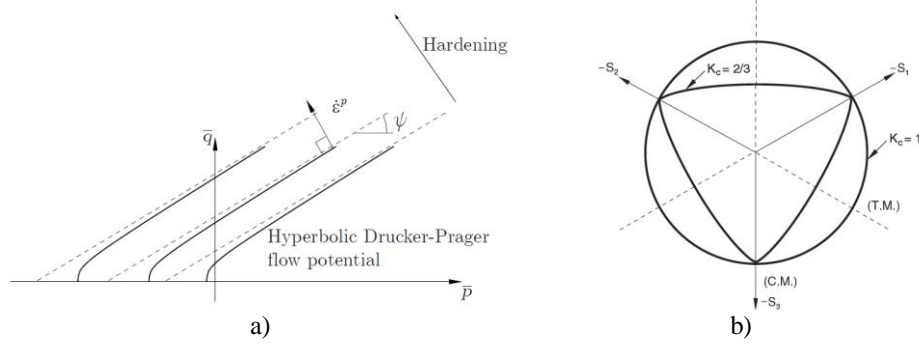
Figure 7: a) Hyperbolic flow potential function; b) Yield function in the deviatoric plane [5].
