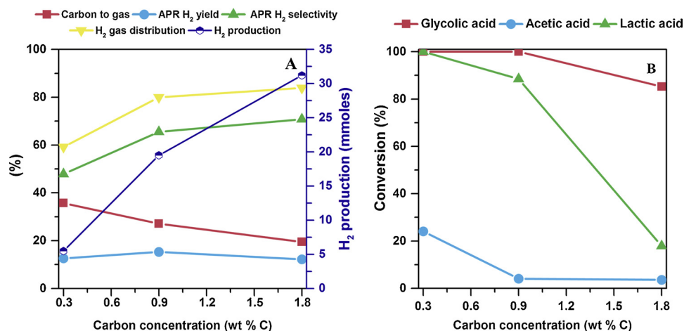
Fig. 5. Influence of carbon concentration on the reaction parameters (A) and conversion (B) of APR of the synthetic mixture. Reaction conditions: liquid phase amount 75 g, reaction temperature 270 °C, reaction time 2 h.
