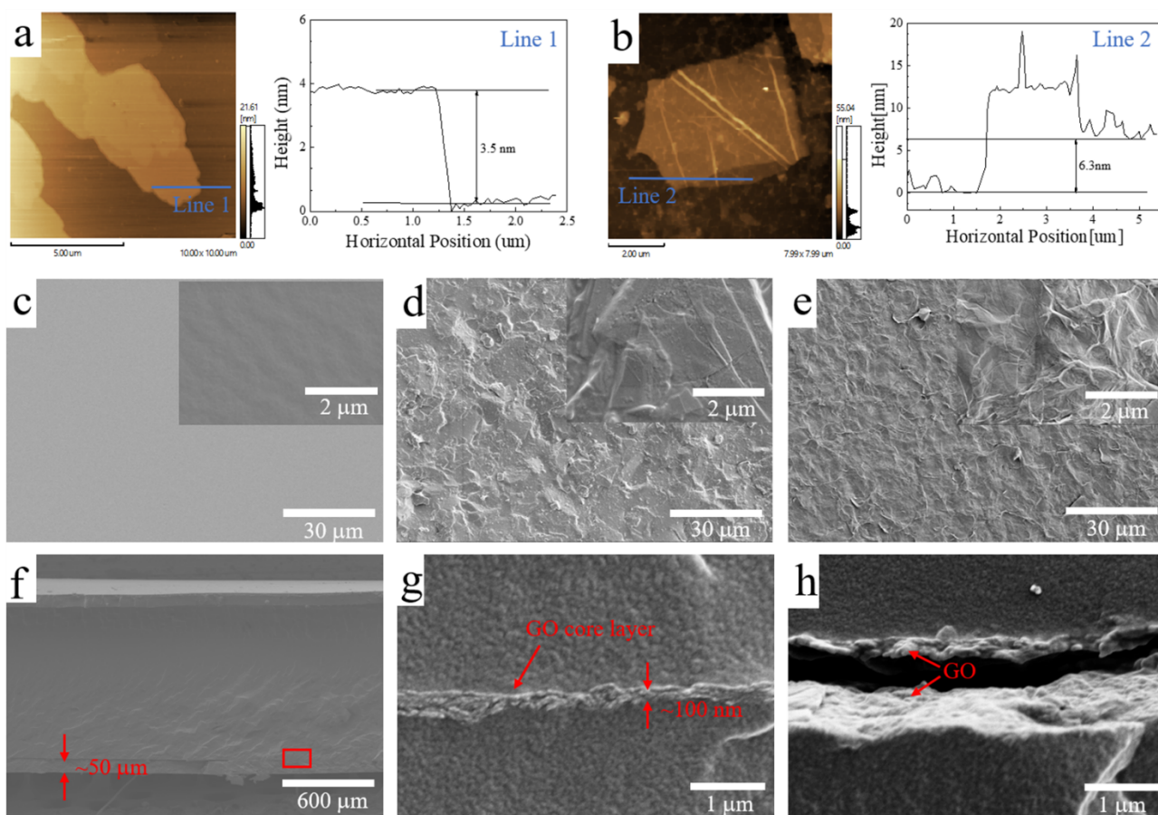
Figure 2. AFM images of as-prepared a) flat GnP and b) wrinkled GO nanoplates and their corresponding height
