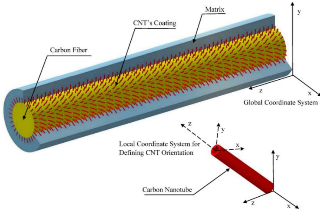
Fig. 7: Schematic illustration of fuzzy fiber reinforced composite RVE with corresponding global and local coordinate systems
