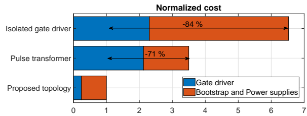
Fig. 17. Comparison between the costs for the different solutions, normalized to the proposed topology.
