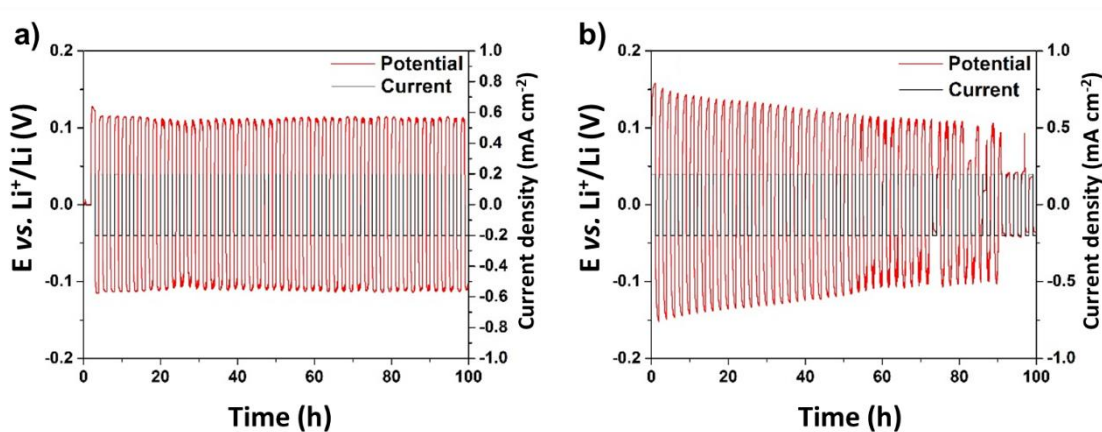
Figure 5. Potential vs. time profiles during the Li plating and stripping experiments carried out in symmetric Li/electrolyte/Li cells assembled with: a) LAGP-free P(EO) 15 LiTFSI, and b) LA-60 all-solid-state electrolytes under study (current density of \pm 0.2 \text{ mA cm}^{-2} fixing each cycle to 1 h at 60 °C).
