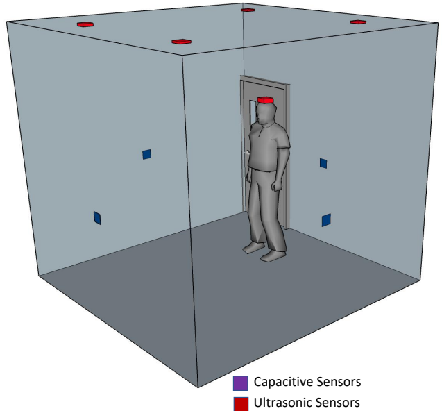
Figure 3: Our 3 m × 3 m experimental room includes one Capacitive sensor on each wall, and five ultrasonic sensors which provide the ground truth (four ultrasonic sensors are on ceiling and one is carried by the monitored person).
