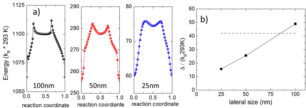
FIG. 3. (a) MEP profile for 100\text{ nm} (black), 50\text{ nm} (red), and 25\text{ nm} (blue) lateral size dots with D = 2\text{ mJ/m}^2 . (b) Thermal stability factor \Delta as a function of the lateral size L estimated at room temperature. The gray dotted line indicates the 42k_B T threshold.
