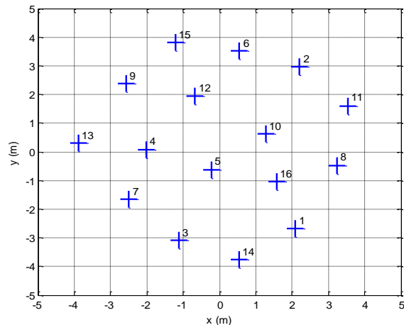
Fig. 2. Array geometry of both AAVS0 and preAAVS1
