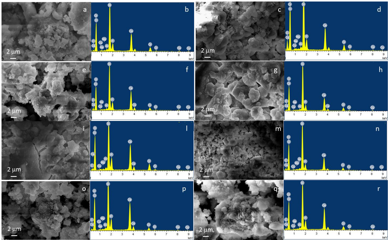
10 11 12 13 14 15 16 17 18 19 20 21 22 23 24 25 26 27 28 29 30 31 32 33 34 35 36 37 38 39 40 41 42 43 44 45 46 47 48 49 50 51 52 53 54 55 56 57 58 59 60 61 62 63 64 65 Figure 10: FESEM-EDS analysis of SBA3-CuUV (a,b), SBA3-CuUV+TT (c,d), SBA3-CuTT (e,f), SBA3-CuUV+TTAr (g,h), SBA3-CuTTAr (i,l), SBA3-CuTA (m,n), SBA3-CuAA (o,p), SBA3-CuNaOH (q,r) after 14 days of immersion in SBF solution.
