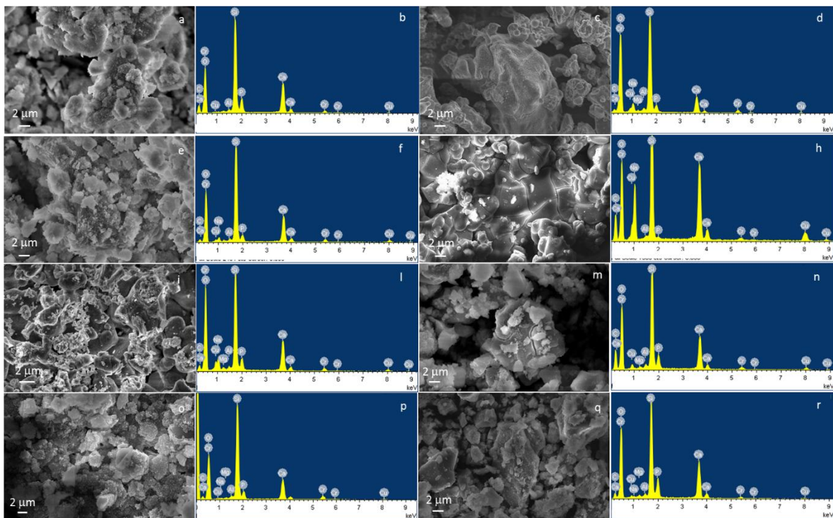
Figure 8: FESEM-EDS analysis of SBA3-CuUV (a,b), SBA3-CuUV+TT (c,d), SBA3-CuTT (e,f), SBA3-CuUV+TTAr (g,h), SBA3-CuTTAr (i,l), SBA3-CuTA (m,n), SBA3-CuAA (o,p), SBA3-CuNaOH (q,r) after 3 days of immersion in SBF
