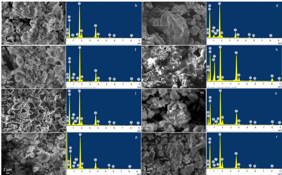
48 49 50 51 52 53 Figure 8: FESEM-EDS analysis of SBA3-CuUV (a,b), SBA3-CuUV+TT (c,d), SBA3-CuTT (e,f), SBA3-CuUV+TTAr (g,h), SBA3-CuTTAr (i,l), SBA3-CuTA (m,n), SBA3-CuAA (o,p), SBA3-CuNaOH (q,r) after 3 days of immersion in SBF
