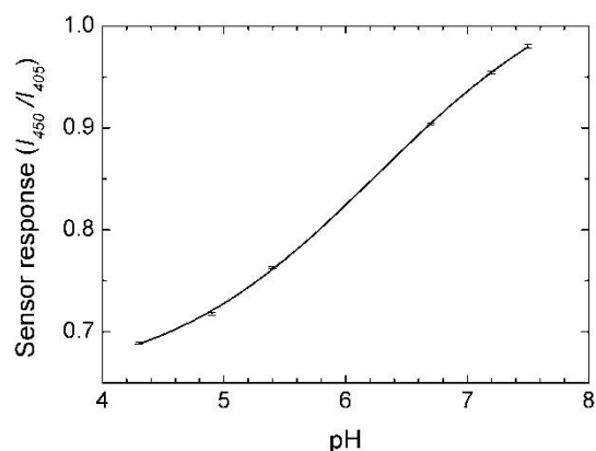
Figure 2. Optical fiber pH sensor response in the wavelength range between 5 and 7 (fitted by Boltzmann's equation).
