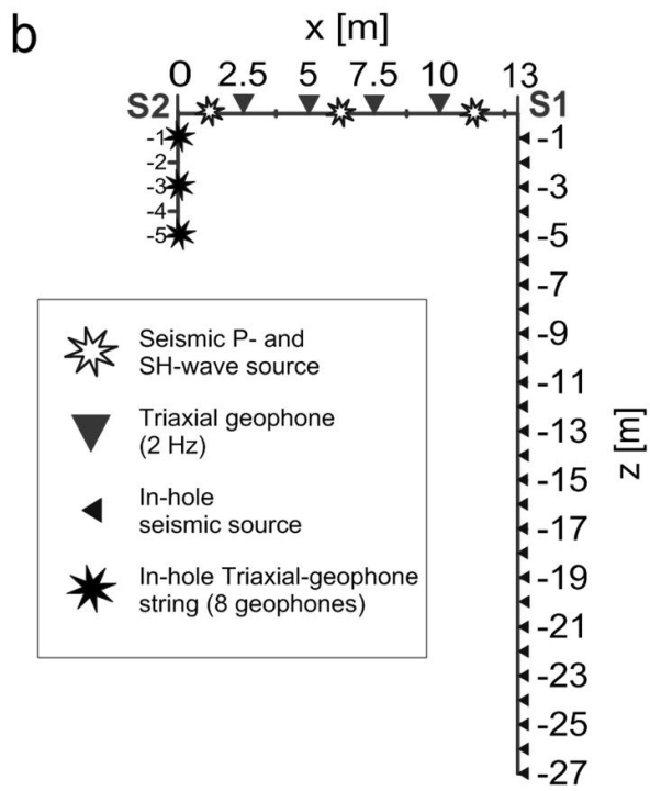
Figure 2. Sketch of the front yard of Madonna del Sasso site, in which the main traces of the fracture systems and the inclinometric boreholes positions are reported (a). Acquisition scheme for the cross-hole seismic tomography survey (b).
