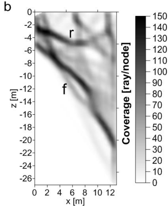
Figure 3. Results of the cross-hole seismic tomography for P waves: velocity (a) and ray coverage (b) sections.
