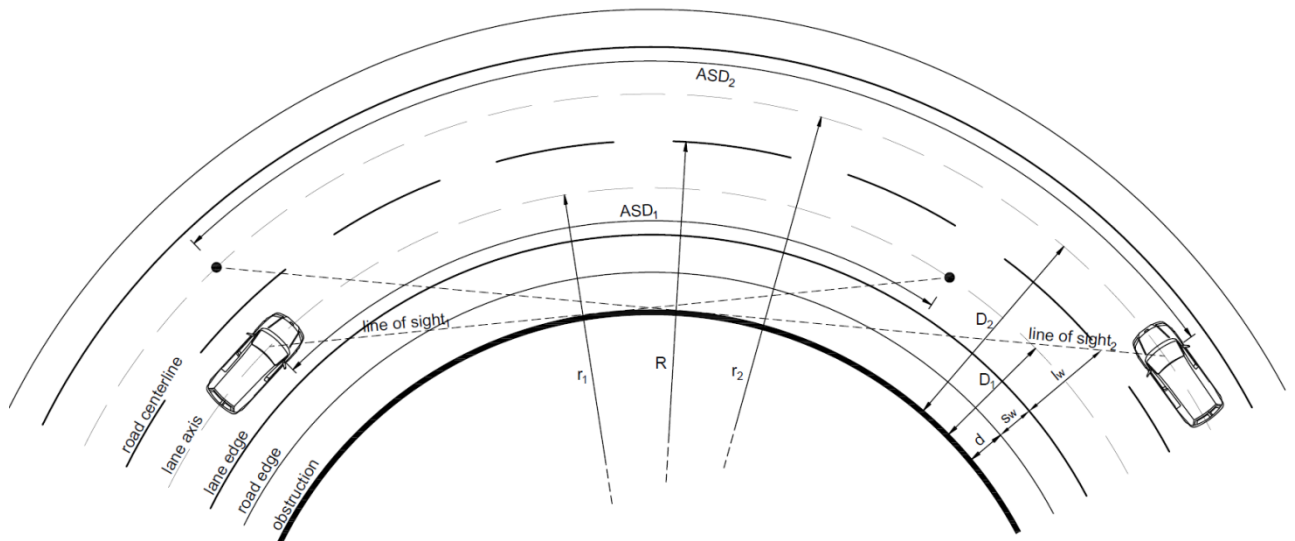
180 Figure 1. Conventional available sight distance (ASD) along a horizontal curve elaborated from road geometric policies 181 (AASHTO, 2011; MIT, 2001). In the figure: R is the radius of the road axis; r_1 and r_2 are the radii of the right- and leftward 182 turn trajectories respectively; D_1 and D_2 are the offsets of sight obstruction from the right- and leftward trajectories 183 respectively; d is the distance of sight obstruction from the road edge; s_w is the shoulder width; ASD_1 and ASD_2 are the 184 available sight distances from the right- and leftward trajectories respectively. 185 186
