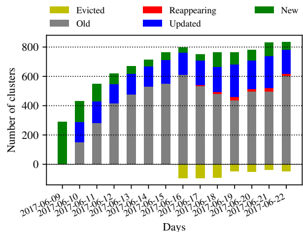
Figure 9: Daily enhancement of system knowledge in HTTPS traces.
