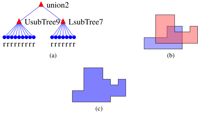
Fig. 3. An illustration of how union2 sub-tree work
