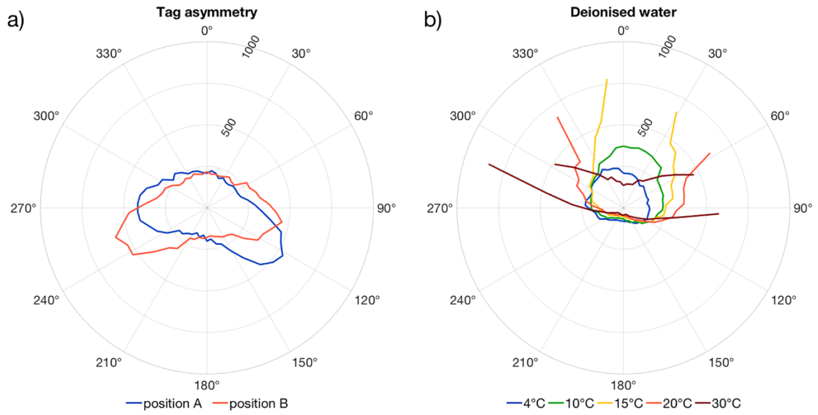
Fig. 3. a) P_{\min} [mW] for activation of the tag when attached to an HDPE flask containing a solution of sodium chloride (0.2%) in position A and by reversing tag position by a 180° plane rotation around tag IC (position B). b) P_{\min} [mW] for activation of the tag attached to a HDPE flask filled with deionised water at different temperatures.
