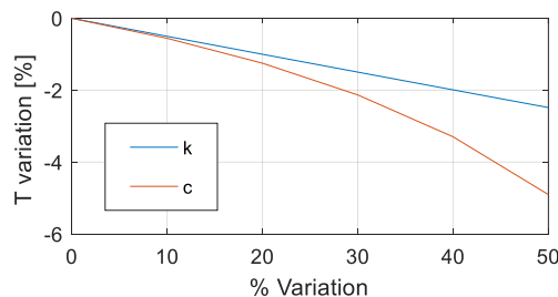
Fig. 9 Indoor temperature variation after 1 hour varying c and k
