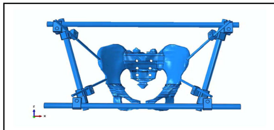
Fig 2.Complete CAD solid model
