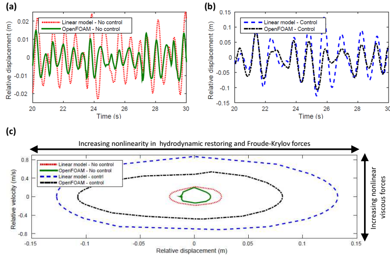
Fig. 6 The relative displacement between the WEC and FSE for (a) the uncontrolled WECs, and (b) the controlled WECs. (c) the relative displacement - relative velocity operational space spanned by the WEC trajectory.
