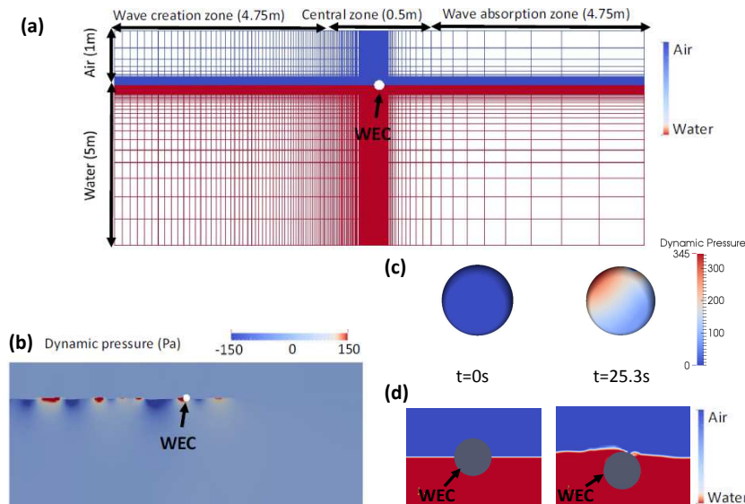
Fig. 2 Cross sectional view of (a) the mesh and fluid volume fractions (water=red, air=blue) at time = 0s, (b) the dynamic pressure at time = 25.3s, (c) the dynamic pressure on the WEC at time = 0s and 25.3s, and (d) the fluid volume fractions around the WEC at time = 0s and 25.3s.
