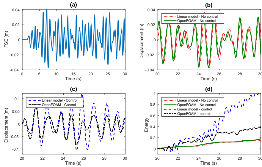
Fig. 4 (a) The measured FSE. (b) the heave displacement for the case of a passive damping PTO. (c) the heave displacement for the case of PI controlled PTO. (d) normalised energy absorbed by the WEC.
