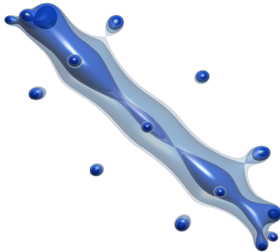
FIGURE 3. Several lemniscates of a perturbation of the configuration for r = 15 constructed with the method of this section.
