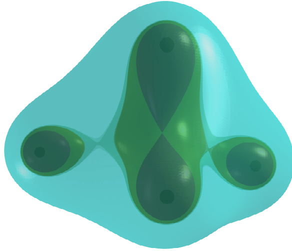
FIGURE 1. A generic big lemniscate configuration for r = 4 surrounded by a non singular level set. The four points are still visible at the interior of the lemniscates.
