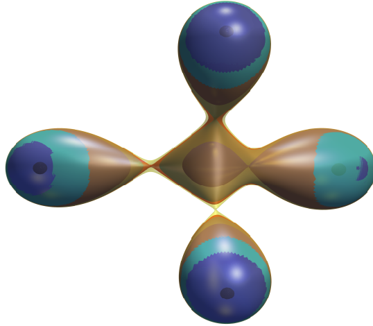
FIGURE 2. Another generic big lemniscate configuration for r = 4 .
