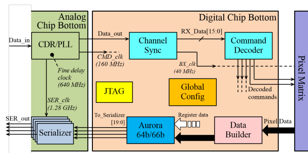
Figure 3: Block diagram of RD53A digital chip bottom.
