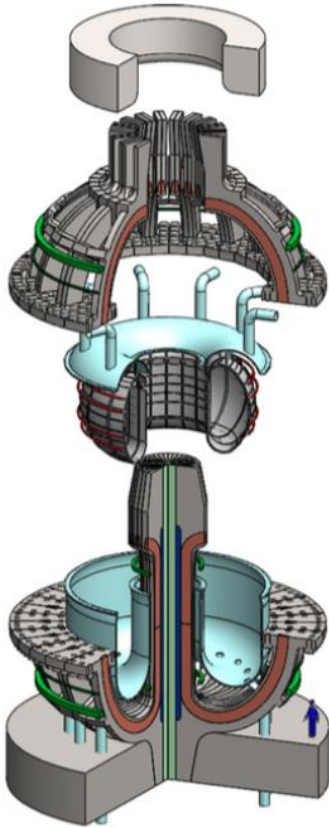
Figure 3 - ARC assembling scheme (Sorbo et al., 2015).
