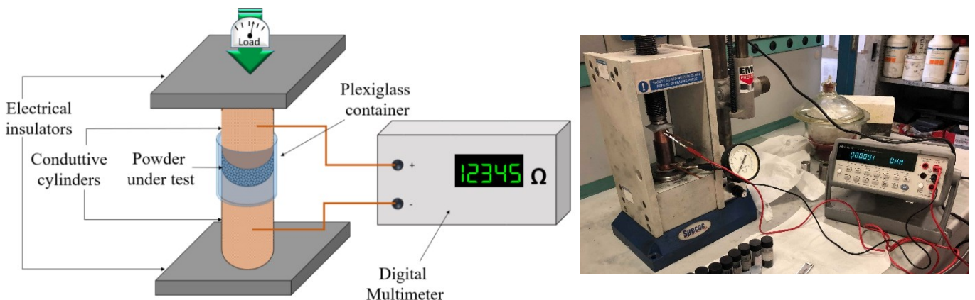
18 Fig. 1. Sketch of Measurement set-up for conductivity study of Biochar powders (left). Measurement set-up 19 for the DC conductivity (right).
