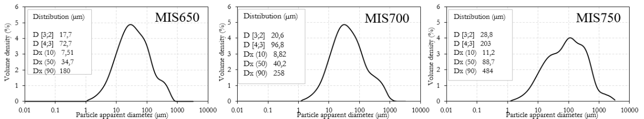
9 Fig. 4 Particle size distribution for MIS650, MIS700 and MIS750
