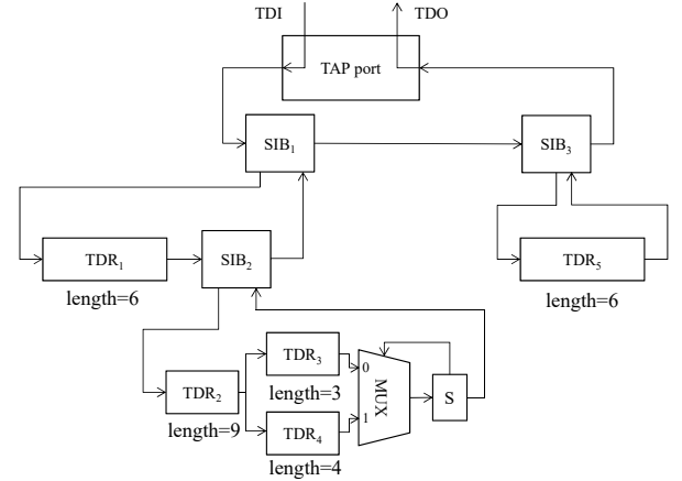
Fig. 3. Example of an IEEE 1687 RSN.
