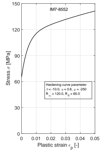
Figure 3. Hardening curve for three laminate systems with curve parameters
