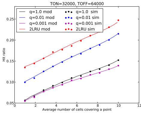
Fig. 5. Trefoil: results for the lazy update rule and an ON-OFF request process with \mathbb{E}[T_f^{ON}] = 3.2 \times 10^4 and \mathbb{E}[T_f^{OFF}] = 6.4 \times 10^4 . The cell request rate for the most popular content is \Lambda = 1.3 .
