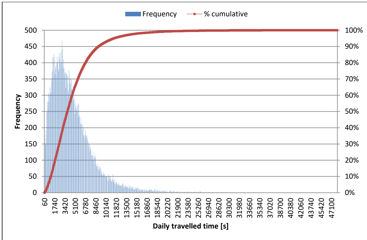
Figure 11: Frequency [#days] of the travel time for all the driving cycles (contexts) and for all the trips.
