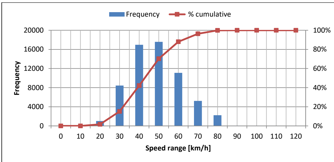
Figure 15: Frequency [# trips] of the average Italian speed in an urban context.
