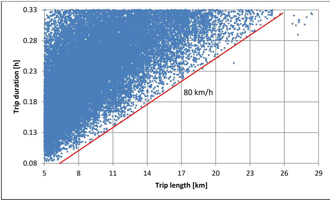
Figure 14: Average speed of Italian extra-urban trips.
