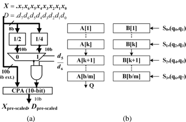
Fig. 4 Example of (a) Scaling Unit (SU) (b) On-the-fly conversion for r=4, t=2 [20]
