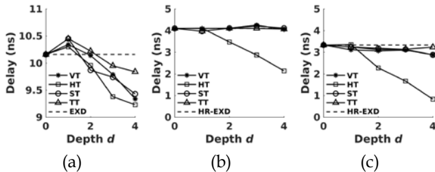
Fig. 29 Delay of 12-bit Approximate Divider with Truncation scheme (a) Radix-2 [18] (b) Radix-4 (c) Radix-8
