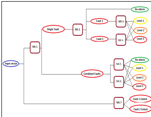
Figure 11. Proposed FDI prognostic algorithm.
