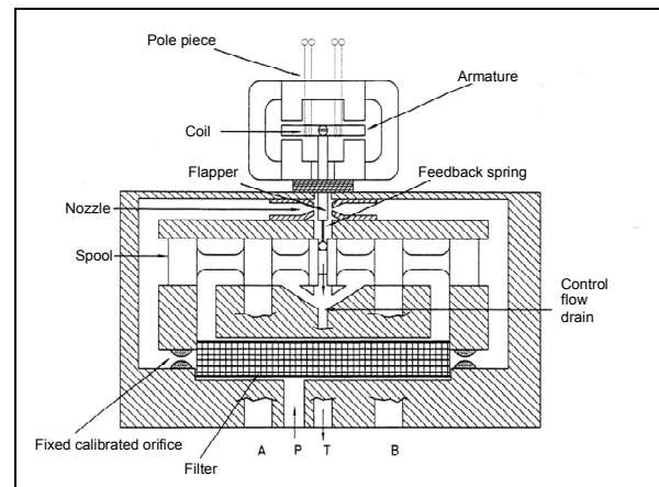
Figure 2. Schematic of the flapper-nozzle servo-valve.
