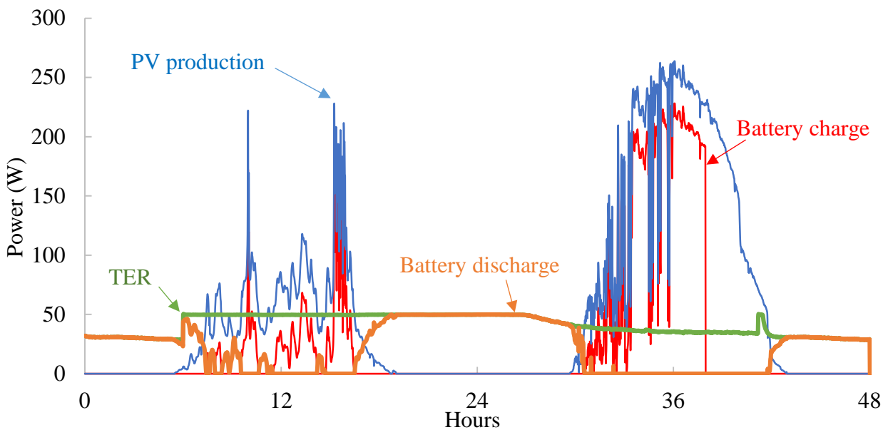
Fig. 18. Power profiles in two days of simulation (10th and 11th day)
