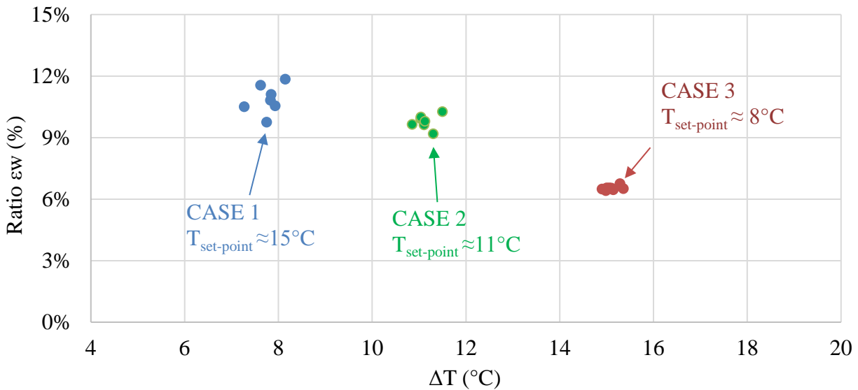
Fig. 10. Chart of temperature difference \Delta T versus the ratio \varepsilon_w ( T_{\text{external}} = 23 \pm 0.5^\circ\text{C} )
