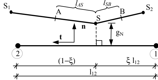
Figure 2: Area of competence of a slave node S and NTS geometry.
