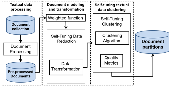
Figure 1: PASTA architecture
