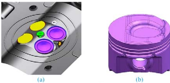
Figure 1. Combustion chamber of the developed NG engine: (a) cylinder head; (b) piston
