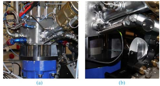
Figure 2. Planar LIF experimental setup: (a) optical single-cylinder engine; (b) last lens used to couple the light sheet from the intake side
