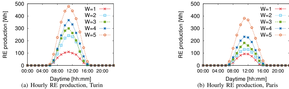
Fig. 7. Hourly energy production of a 1 kW peak PV panel, per each day-type in Turin and Paris, for N_W=5 with equal-probability discretization.
