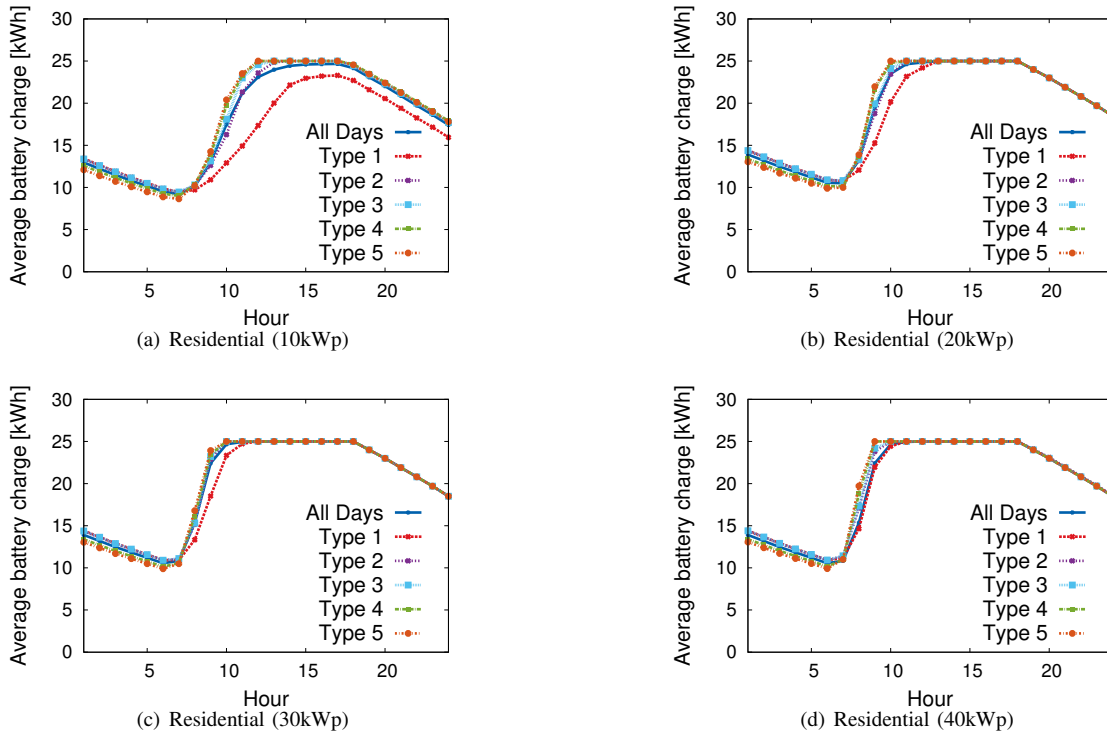
Fig. 21. Average hourly battery charge for a macro BS in Maiduguri versus time, with N_W = 5 and equal-probability discretization, time slot \Delta T = 1h , PV panel sizes 10, 20, 30, and 40 kWp, C_B = 25 kWh, and Q_S = 100Wh (50Wh in case of PV panel size 10 kW peak), for the residential weekday traffic profiles, adopting the EARTH model.
