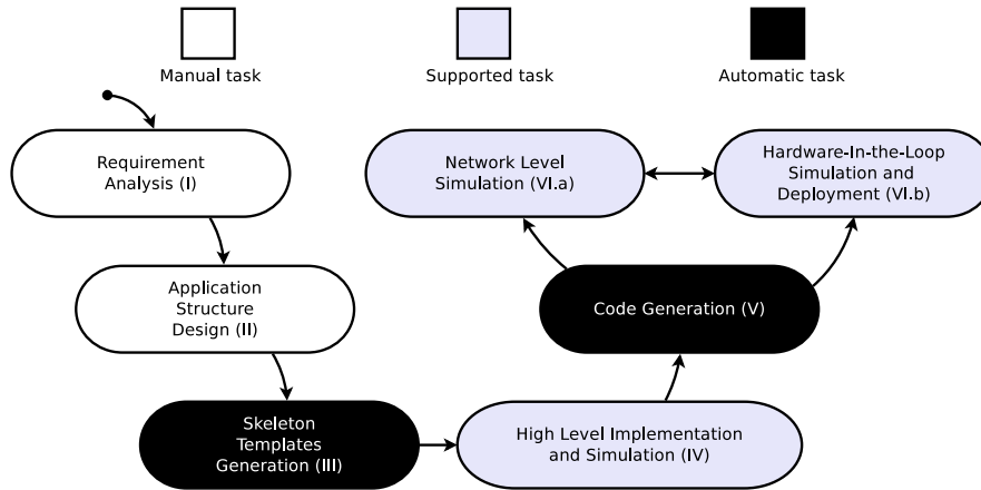
Figure 38.5: Framework development flow is based on a V-shape iterative model.
