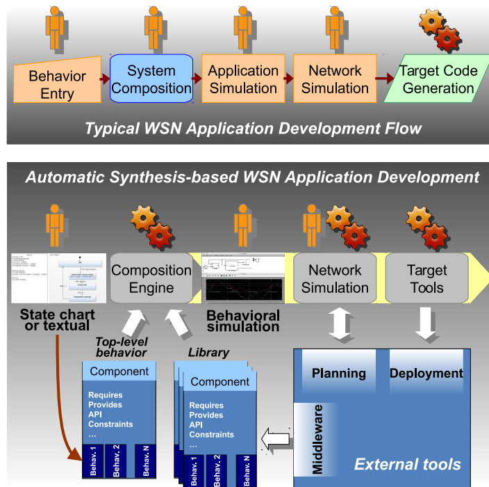
Figure 38.10: Comparison of the main stages of manual (top) and automated (lower part) node-level WSN application design flows. A human body tags manual phases while a gear tags automatic ones. The automated flow accelerates mainly the system composition and the preparation of the network simulation.
