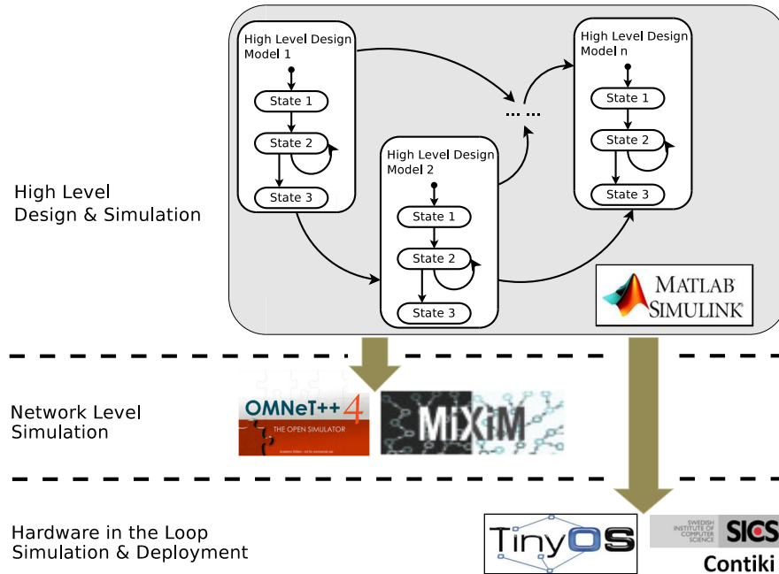
Figure 38.2: Overview of the development flow based on Simulink ® framework.
