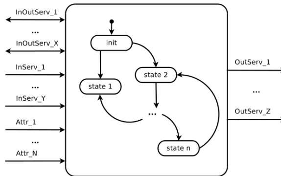
Figure 38.4 A StateChart implements a finite state machine which defines the behavior of a functional module.
