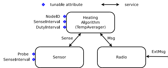
Figure 38.8 Module structure of example node-level WSN application.
