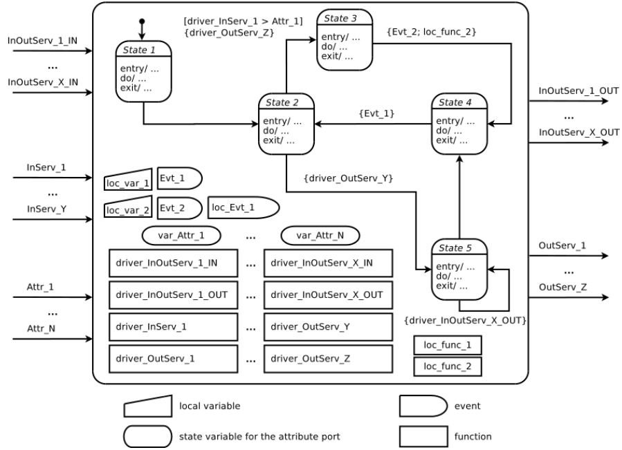
Figure 38.7: Example of complete WSN node application skeleton.
