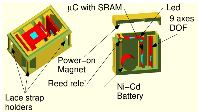
Fig. 3. The sensor assembly: the sealed box which contains the IMU, the Teensyduino microcontroller, the \mu Panel wireless board, the power on reed relé and the magnet, the NiCd battery and the led for the user feedback.
