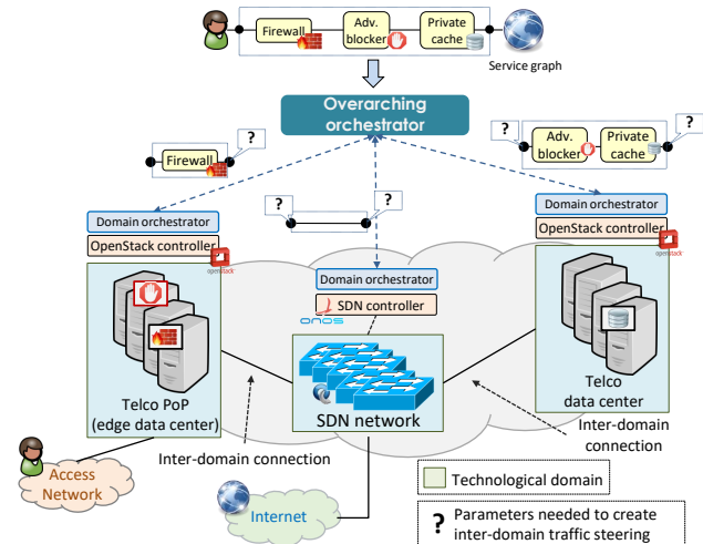
Fig. 1. Service graph deployment in a multi-domain environment.
