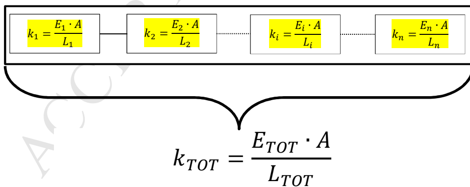
Figure 6: Mechanical model of a damaged specimen subjected to a longitudinal load.
