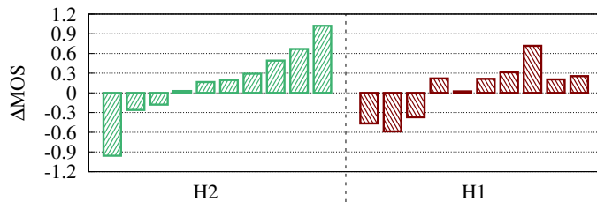
Fig. 6: \Delta MOS for 10 pages where we contrast unsharded vs sharded versions.
