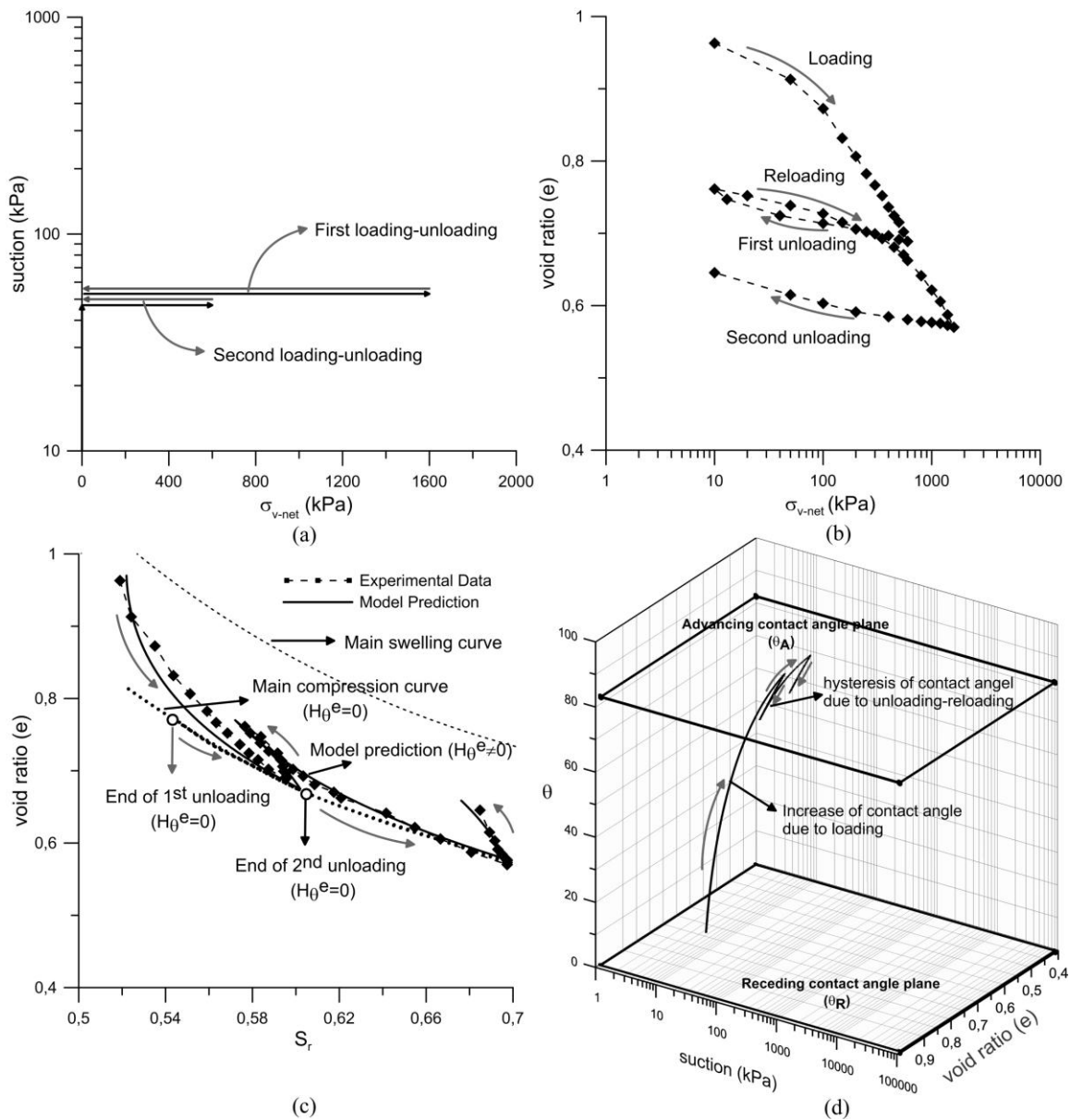
Figure 6. Computed and experimental behaviour during loading–unloading cycles at constant suction (a) applied loading path (b) void ratio-net stress data(c) void ratio-degree of saturation data and predictions (d) evolution of the contact angle with suction and void ratio.
