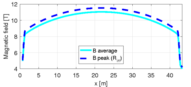
Fig. 3. Distribution of the magnetic field amplitude (left axis), on the cable axis and at the conductor inner radius, in SULTAN-like conditions [10].
