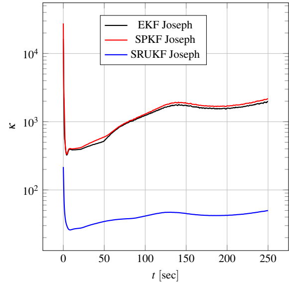
Fig. 9 Condition Number of the state covariance matrix \mathbf{P}^{xx}_{n/n} using Joseph formulation for EKF and UKF and of \mathbf{S}^{xx}_{n/n} using Joseph formulation for SRUKF from 500 Monte Carlo runs
