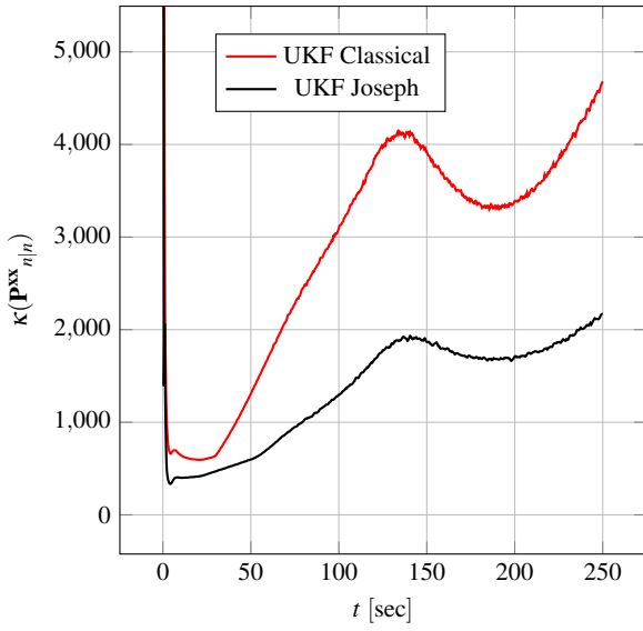
Fig. 7 Condition Number of the state covariance matrix \mathbf{P}^{xx}_{n/n} for the UKF using classical and Joseph formulation from 500 Monte Carlo runs
