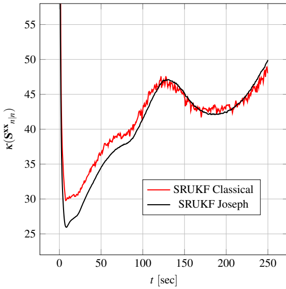
Fig. 8 Condition Number of \mathbf{S}^{xx}_{n/n} for the SRUKF using classical and Joseph formulation from 500 Monte Carlo runs
