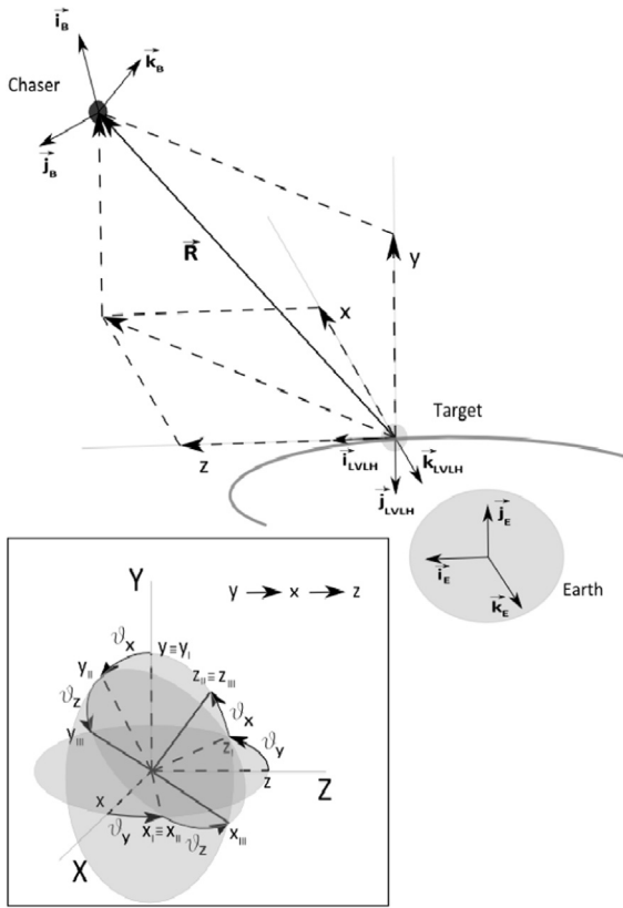
Fig. 1. Vectorial representation of the chaser position with respect to the target, including the inertial frame E , the local vertical local horizontal frame LVLH and the body frame B ; attitude representation through the Euler angles parametrization, according to the sequence yxz (box).
