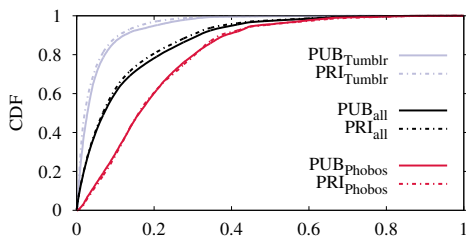
(a) Download CDFs for flows carrying \geq 1 MB.
