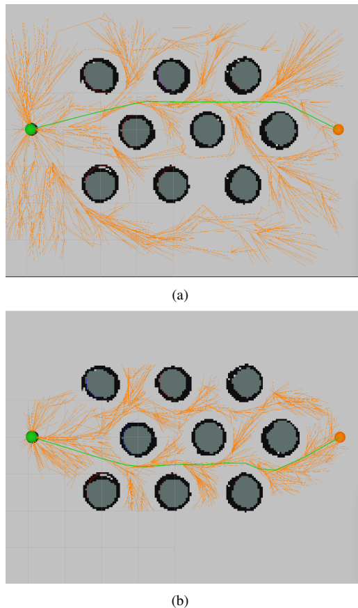
Figure 6. An example where we simulate a planning problem. In both figures the start and goal points, as well as the statics environment, are the same; the solution time is 0.5 seconds for both methods. Figure (a) shows the RRT* solution, while in (b) the same solution obtained with Informed-RRT* is presented. The solution path is represented in green, the exploration tree in orange. Notice that Informed-RRT* uses Search-Space more efficiently, while RRT* continues to use the entire Space. After 0.5 seconds both algorithms find a near-optimal solution.
