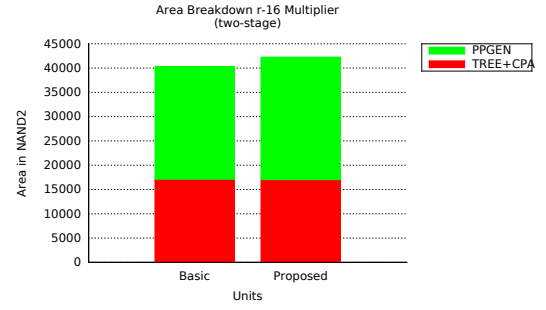
Fig. 9. Area breakdown for 2-stage pipelined multipliers.
